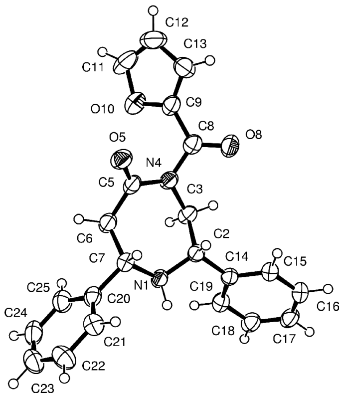
Figure 1 View of the asymmetric unit of the title compound, showing the atom-labelling scheme. Displacement ellipsoids are drawn at the 50% probability level and H atoms are represented by circles of arbitrary radii.
