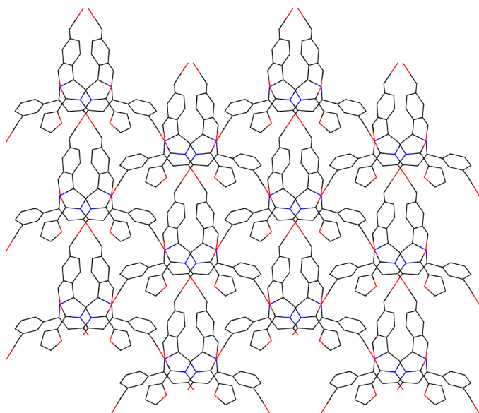
Figure 2 Part of the crystal structure, showing the supramolecular aggregation through weak C—H...O intermolecular interactions.
